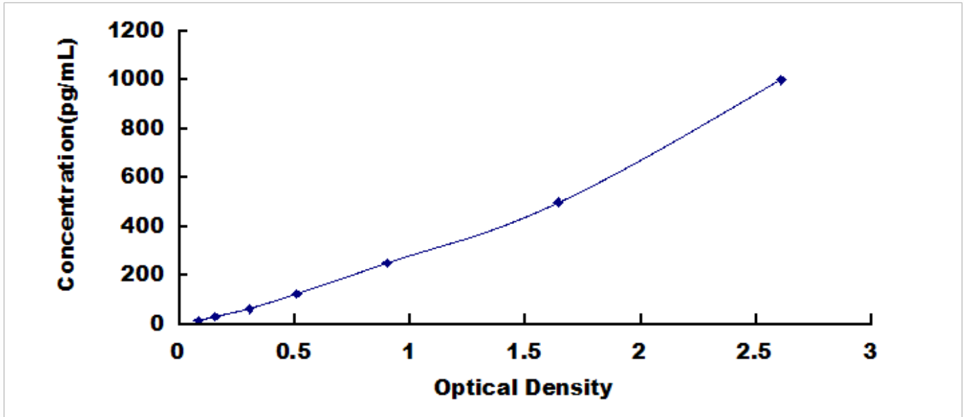
Typical Standard Curve for MCP1, Rabbit ELISA.
